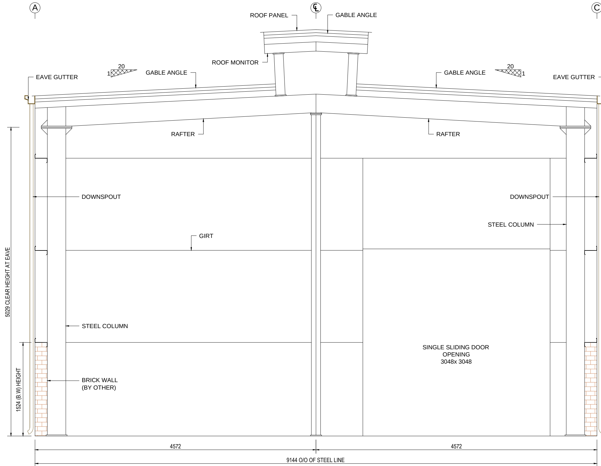
END WALL FRAMING @ GRID-1
